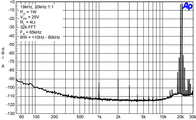
Intermodulation Distortion
