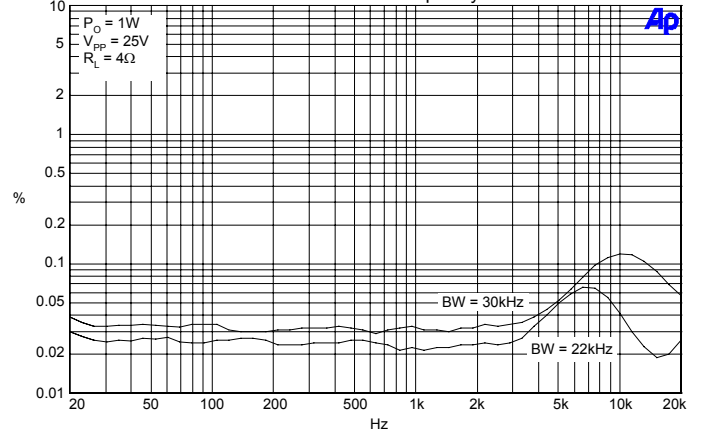
THD+N versus Frequency
